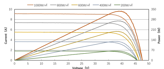
I-V & P-V curve AE DGM6-72
